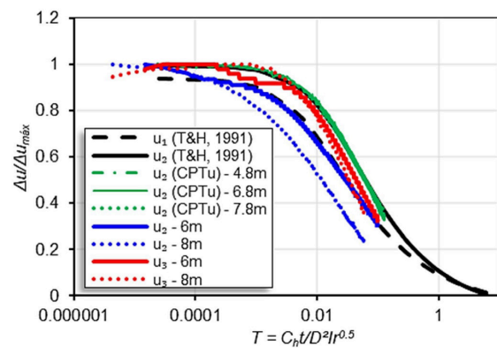
Figure 8. Excess pore pressure normalized versus time factor: Teh & Houlsby (1991) proposal.
