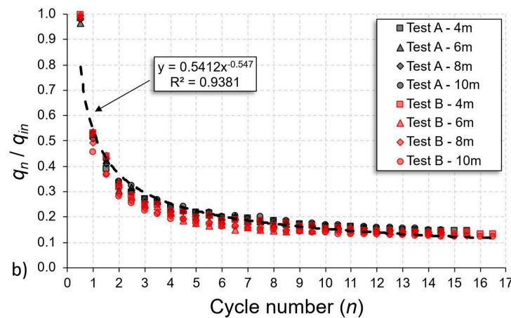
Figure 6. Cycling test analysis (a) q_n (b) normalized degradation curve – q_n/q_{in} (c) normalized degradation curve q_n/q_{in} and prediction considering Equation 5.
