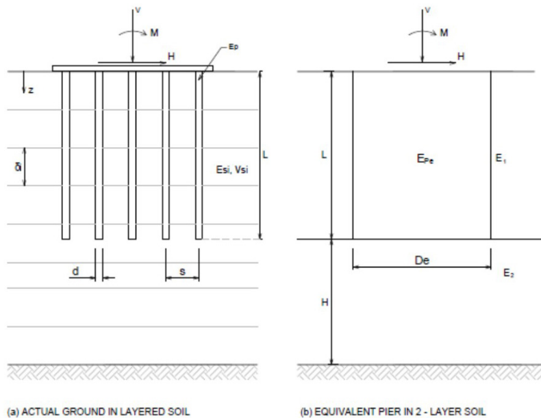
Figure 2. Equivalent pier approximation.
