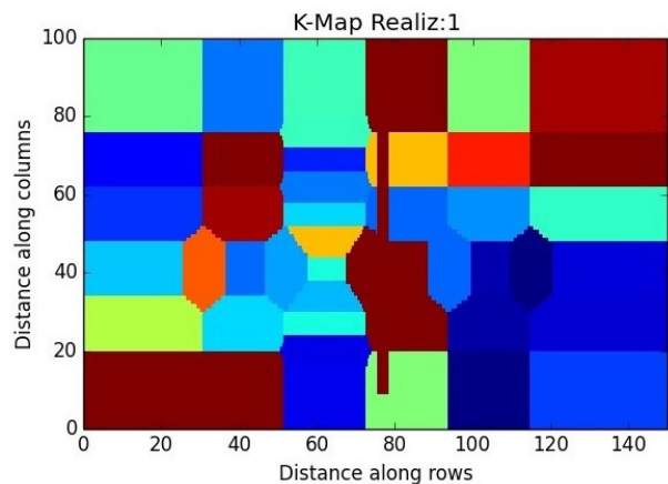
Figure 12. Plan view of the domain with k map based on the nearest-neighbor criterion ( k in m/d, color bar in Figure 10).
