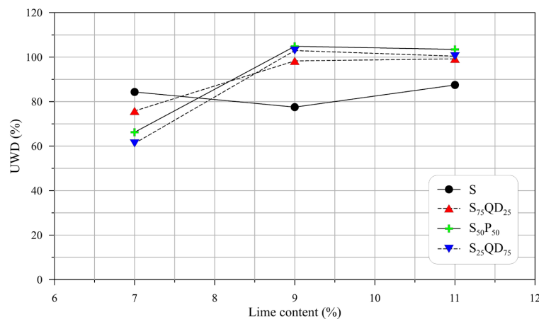
Figure 10. Strength improvement factors (UWD) treated with lime after wetting-drying cycles.
