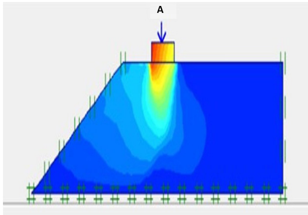
Figure 7. Footing on slope.
