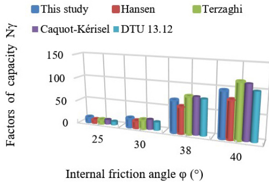
Figure 4. Comparison of N_\gamma values with those available in the literature.
