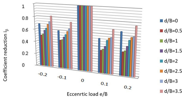
Figure 11. Variation of Reduction factor i_\beta as a function of the ratio of eccentricity e/B .
