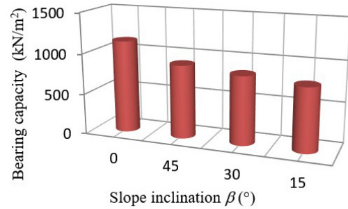
Figure 8. Bearing capacity values of the footing as a function of \beta .
