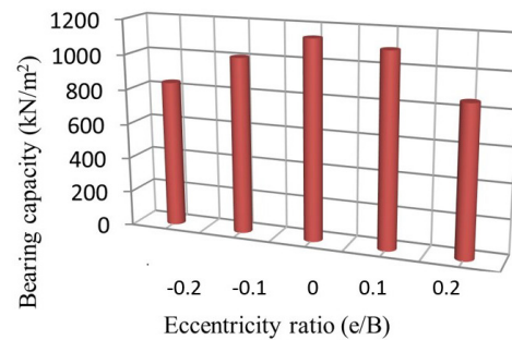
Figure 9. Influence of the load eccentricity on the bearing capacity for \beta = 0^\circ .
