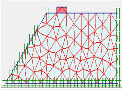
Figure 2. Presentation of the digital model.
