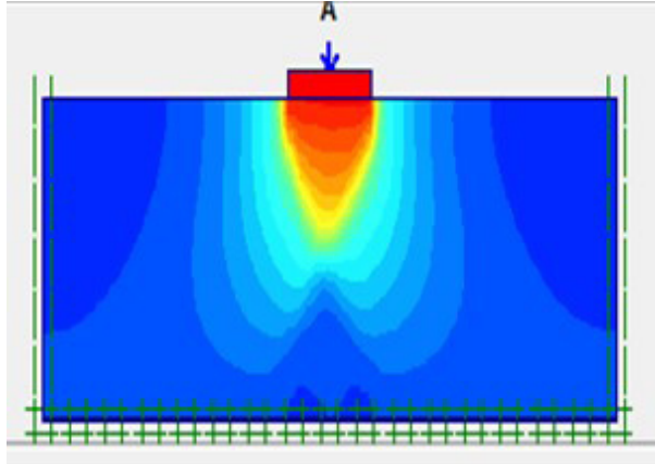
Figure 3. Modeling of a sole on a horizontal surface.
