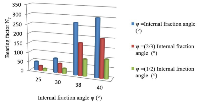
Figure 5. Lift factors as a function of \psi for a horizontal surface.
