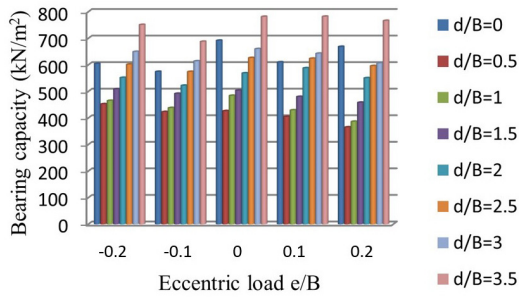
Figure 10. Variation of bearing capacity as a function of the ratio of eccentricity e/B .
