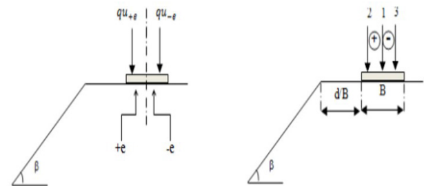
Figure 6. Sign convention (1) centered charge, (2) positive eccentric charge and (3) negative eccentric charge.
