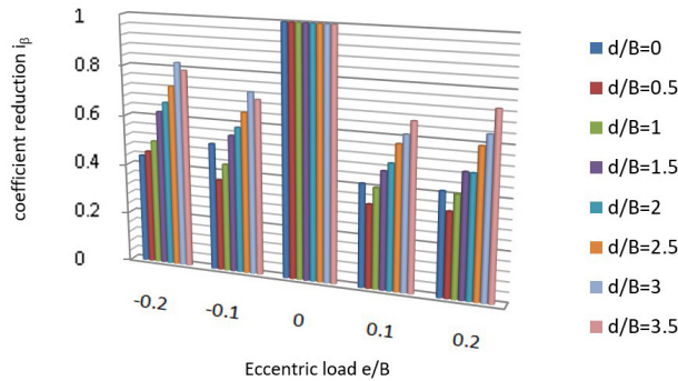
Figure 12. Variation of Reduction factor i_\beta as a function of the ratio of eccentricity e/B .
