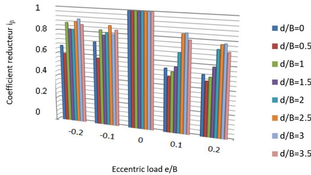
Figure 13. Variation of Reduction factor i_\beta as a function of the ratio of eccentricity e/B .
