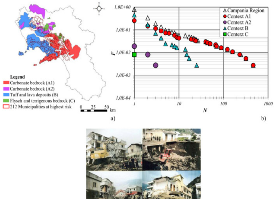
Figure 14. a) The bedrock in the area covered by pyroclastic soils, b) the Societal risk in the area of the pyroclastic soils, examples of damages to properties in the geological context A1 caused by c) the event dated 1998 along the Pizzo d'Alvano massif [modified from Cascini (2004)].
