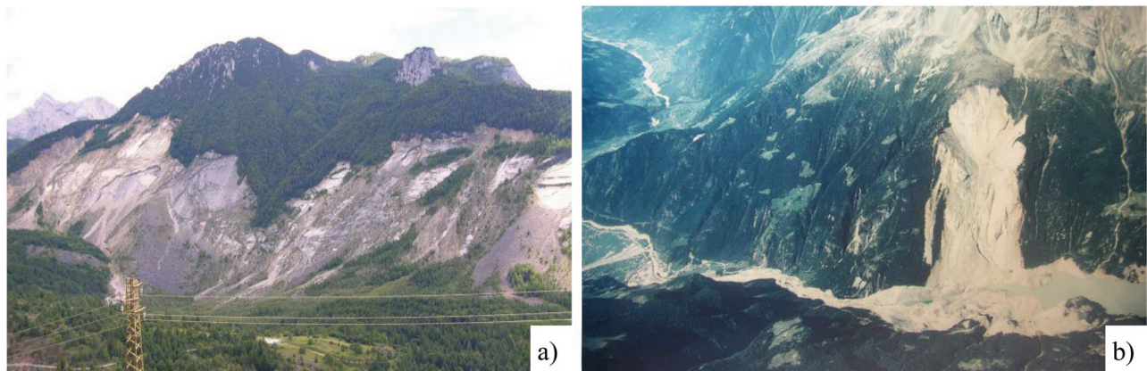
Figure 2. a) Vajont landslide (Wikipedia, 2023); b) Val Pola landslide [Studio Majone Ingegneri Associati (2023)].
