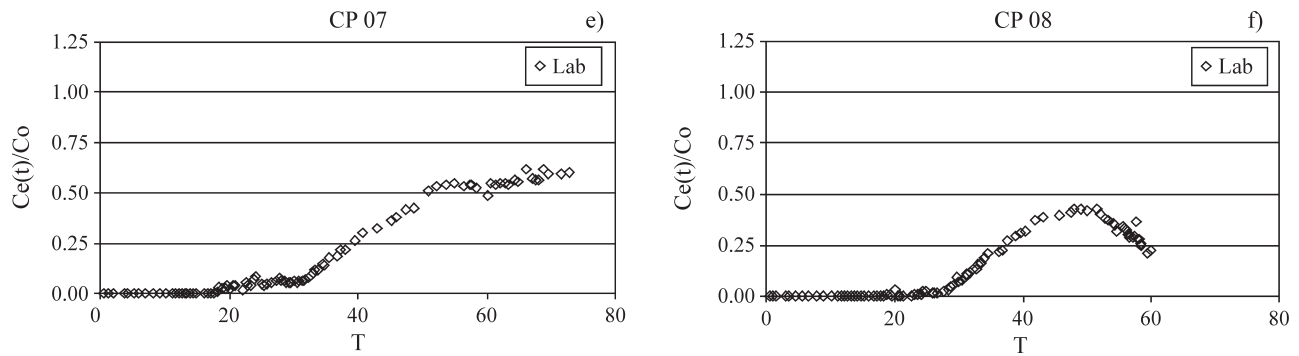
Figure 16 (cont.) - Cadmium elution curves from soil columns: (e) CP07, (f) CP08.
