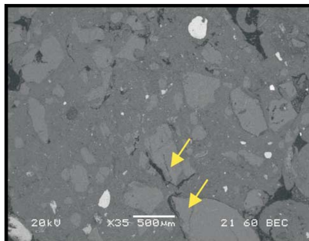
Figure 23 - Few fissures present - CP08.
