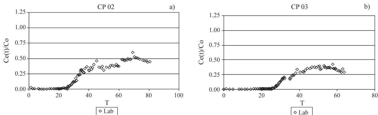
Figure 15 - Zinc elution curves from soil columns: (a) CP02, (b) CP03.
