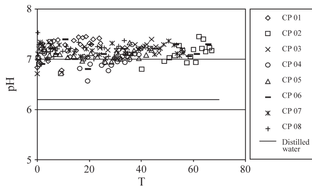
Figure 5 - Leachate pH of soil column percolated with distilled water.
