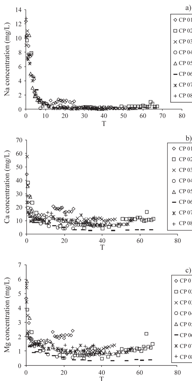
Figure 3 - Cations in soil column leachates percolated with distilled water (a) sodium, (b) calcium, (c) magnesium.
