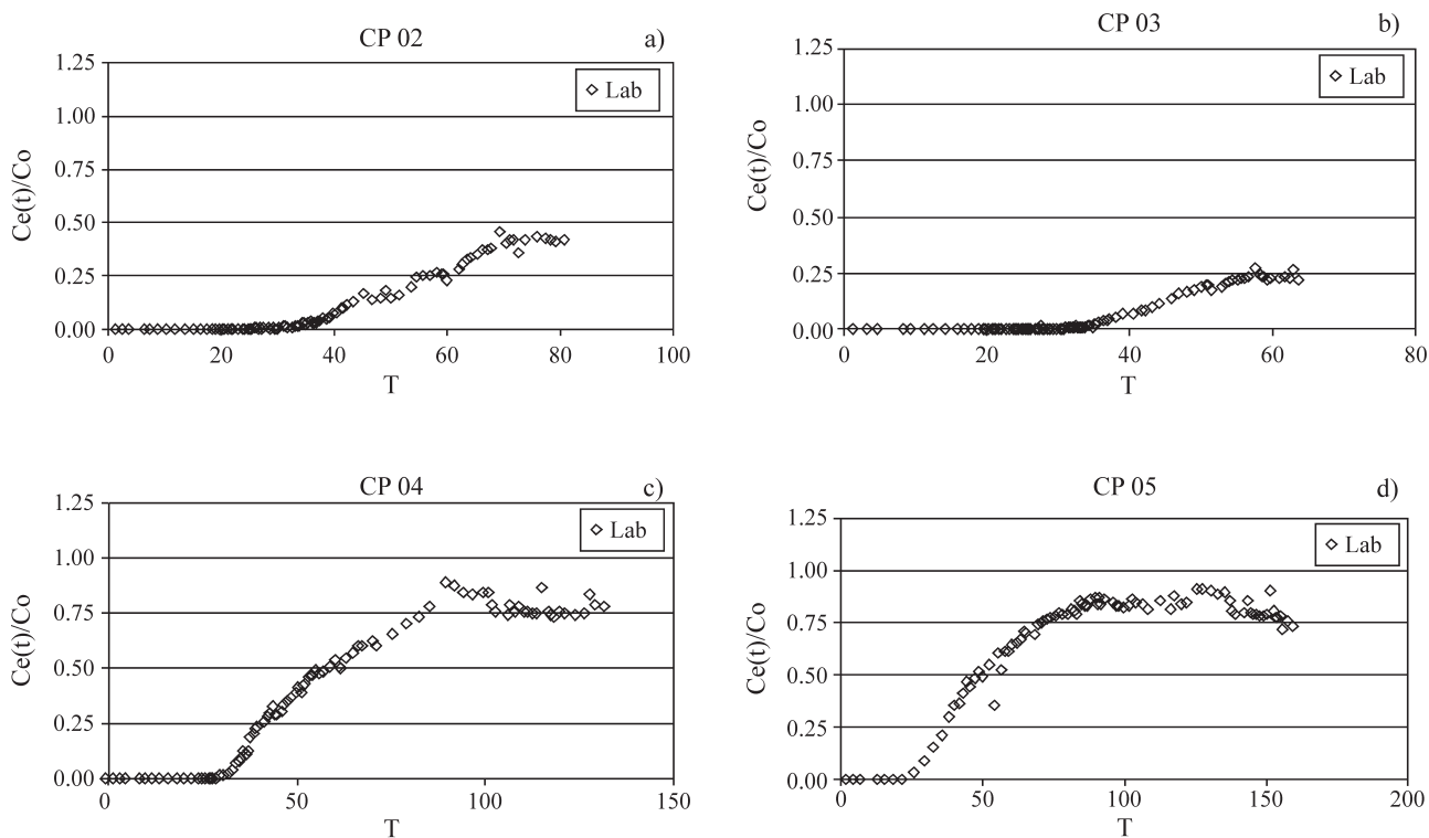
Figure 16 - Cadmium elution curves from soil columns: (a) CP02, (b) CP03, (c) CP04, (d) CP05.
