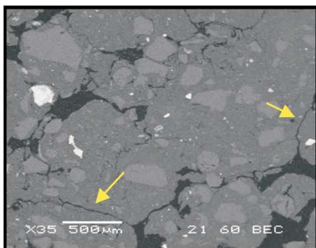
Figure 21 - Few fissures present - CP02.
