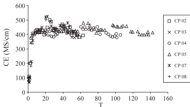
Figure 8 - Electrical conductivity in leachate from soils columns percolated with contaminant solution.
