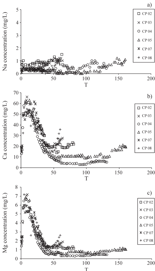
Figure 7 - Cation concentrations concentration in leachates from soil columns percolated with contaminant solution: a) sodium, b) calcium e c) magnesium.
