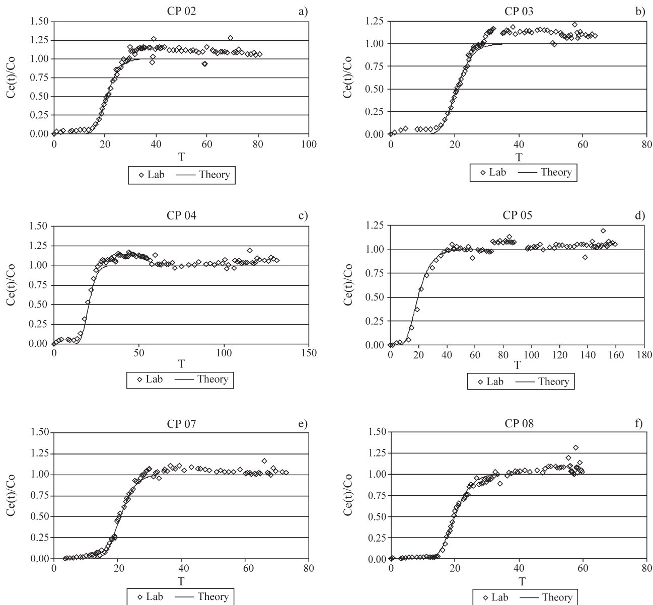
Figure 14 - Manganese elution curves from soil columns: (a) CP02, (b) CP03, (c) CP04, (d) CP05, (e) CP07, (f) CP08.
