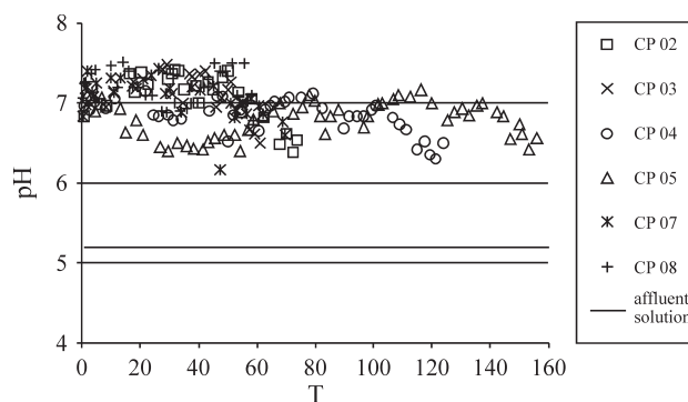
Figure 9 - pH of leachate from soil columns percolated with contaminant solution.
