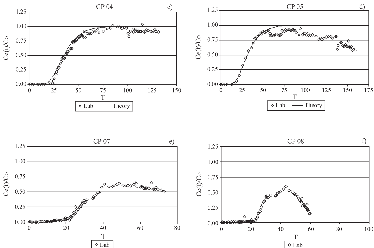
Figure 15 (cont.) - Zinc elution curves from soil columns: (c) CP04, (d) CP05, (e) CP07, (f) CP08.
