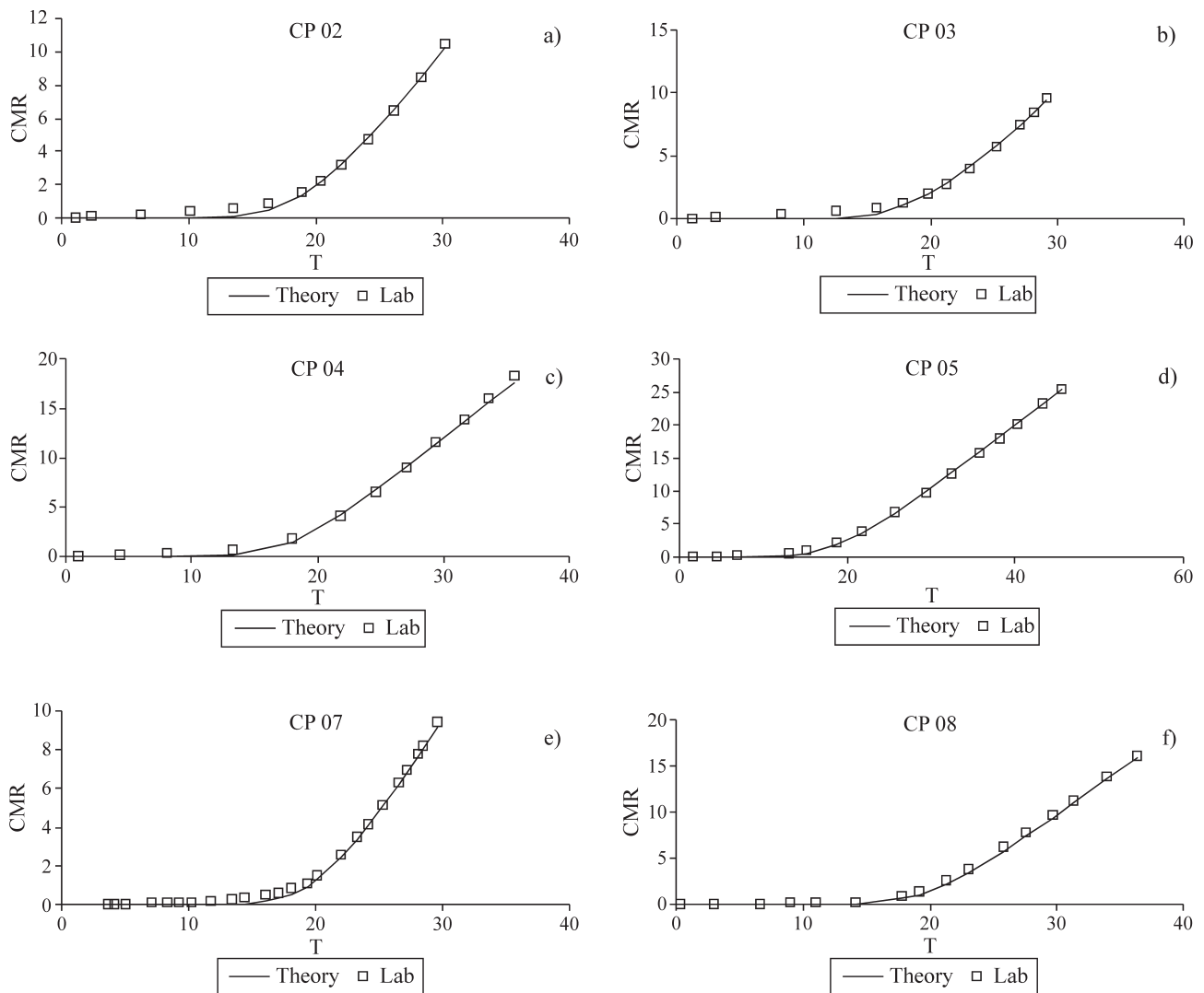
Figure 17 - Manganese cumulative mass ratio curves. CP02, (b) CP03, (c) CP04, (d) CP05, (e) CP07 e (f) CP08.
