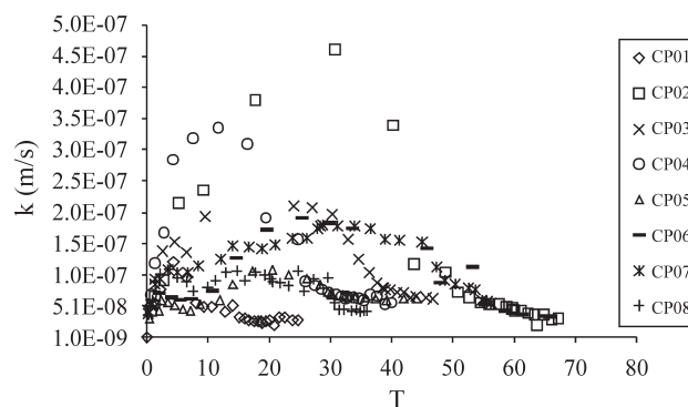
Figure 2 - Hydraulic conductivity in samples percolated with distilled water.
