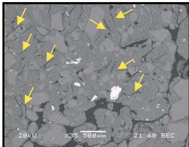
Figure 20 - Various fissures present - CP06.
