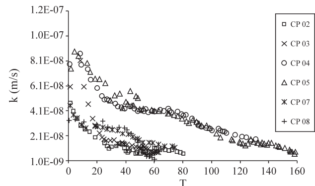
Figure 6 - Hydraulic conductivity in soil samples percolated with contaminant solution.
