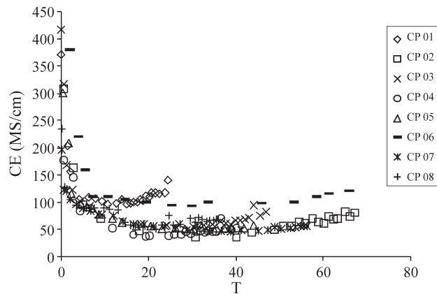
Figure 4 - Electrical conductivity (CE) in soil columns percolated with distilled water.
