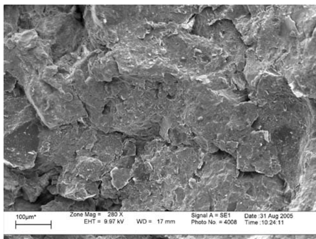
Figure 13 - Microphotograph of sample CP06 (control).
