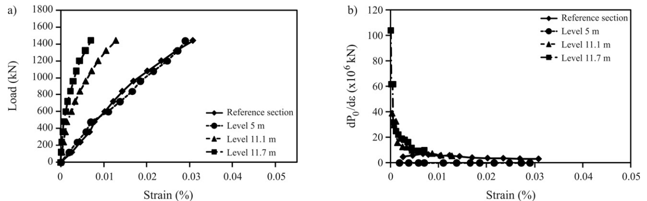
Figure 20 - Results of instrumentation analysis for Omega pile 2.
