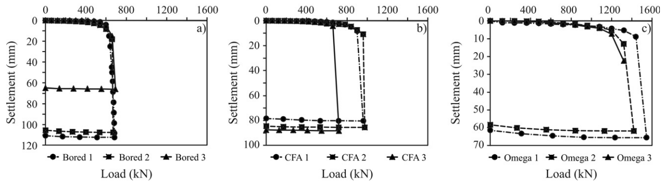
Figure 5 - Load-movement curves.
