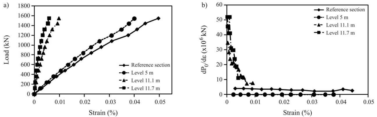
Figure 19 - Results of instrumentation analysis for Omega pile 1.
