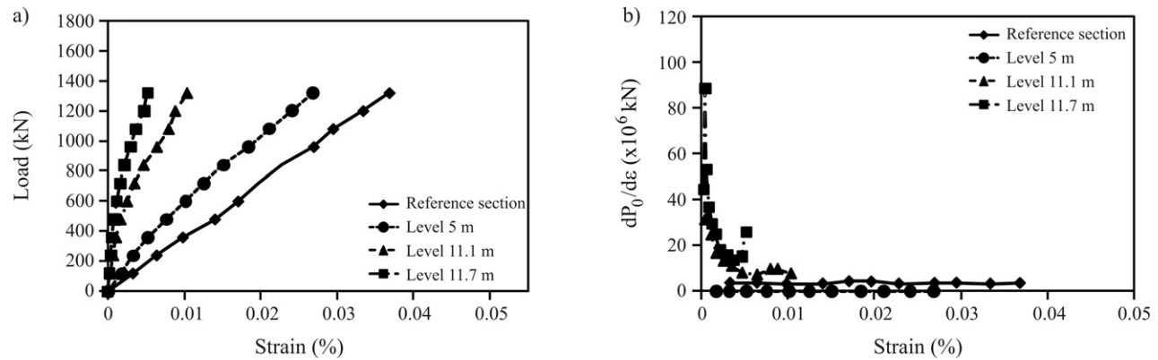
Figure 21 - Results of instrumentation analysis for Omega pile 3.
