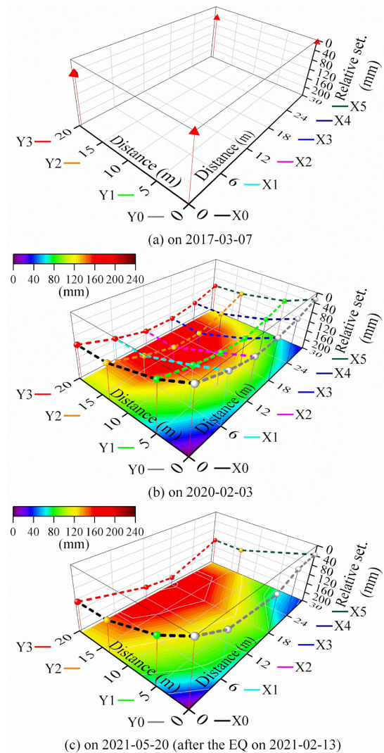
Figure 7. Distribution of measured relative settlements of the TNF.
