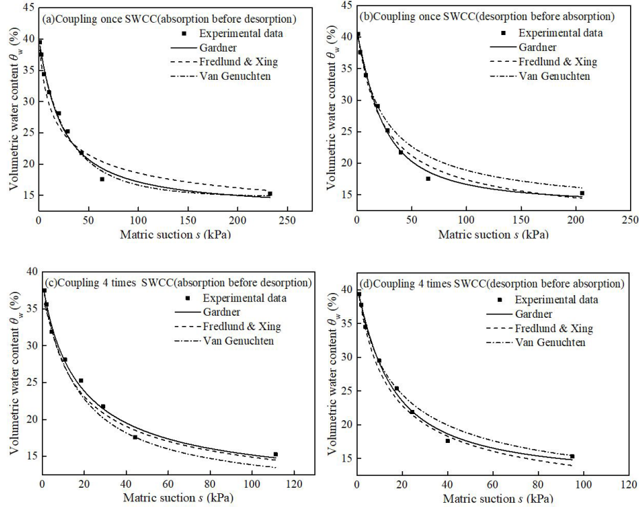
Figure 4. Function fitting for SWCC of different coupling of freeze-thaw and dry-wet: (a) Coupling once and absorption before desorption; (b) Coupling once and desorption before absorption; (c) Coupling 4 times and absorption before desorption; (d) Coupling 4 times and desorption before absorption.
