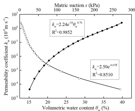
Figure 6. The permeability coefficient function.
