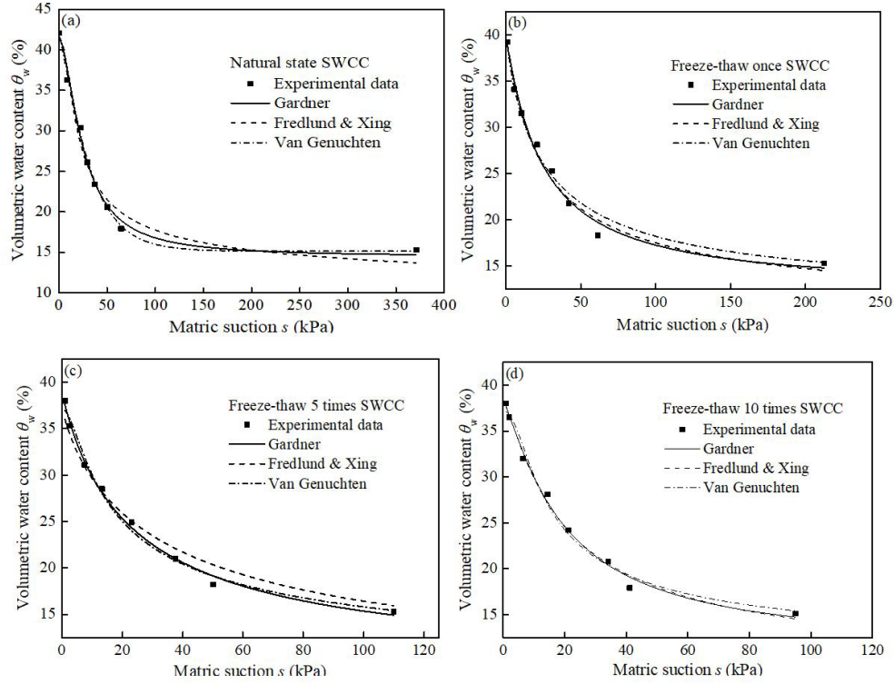
Figure 3. Function fitting for SWCC of different freeze-thaw cycles: (a) Natural state; (b) Freeze-thaw once; (c) Freeze-thaw 5 times; (d) Freeze-thaw 10 times.
