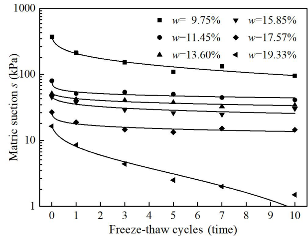
Figure 1. The relation between matric suction and freeze-thaw cycles.
