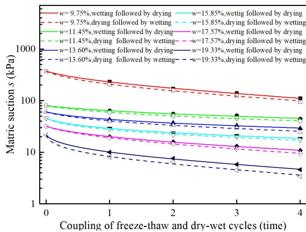
Figure 2. The relation between matric suction and coupling of freeze-thaw and dry-wet.
