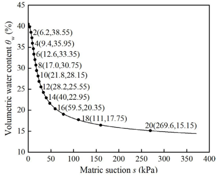
Figure 5. The predicting method of permeability coefficients based on soil-water characteristic curve.
