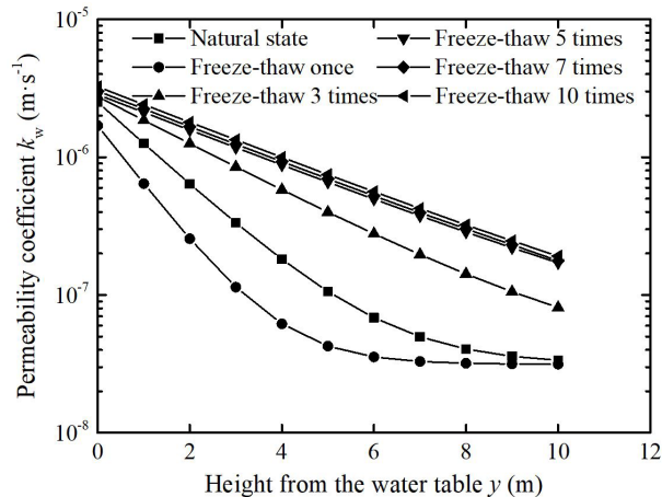
Figure 7. The calculation of vertical permeability coefficient under different conditions.
